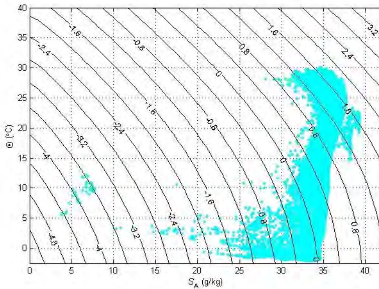
Figure A.14.1. Contours of (|\nabla_n \theta| / |\nabla_n \Theta| - 1) \times 100\% at p = 0 , showing the percentage difference between the epineutral gradients of \theta and \Theta . The blue dots are from the ocean atlas of Gouretski and Koltermann (2004) at p = 0 .
