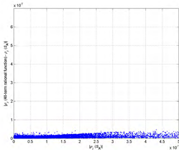
Figure A.30.1. The northward density gradient at constant pressure (the horizontal axis) for data in the world ocean atlas of Couretski and Koltermann (2004) for p > 1000 dbar. The vertical axis is the magnitude of the difference between evaluating the density gradient using the 48-term expression Eqn. (A.30.1) instead of using the full TEOS-10 expression, using Absolute Salinity S_A as the salinity argument in both cases.
