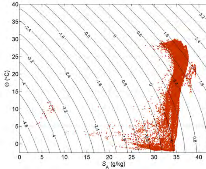
Figure A.14.1. Contours of (|\nabla_n\theta|/|\nabla_n\Theta| - 1) \times 100\% at p = 0 , showing the percentage difference between the epineutral gradients of \theta and \Theta . The red dots are from the ocean atlas of Gouretski and Koltermann (2004) at p = 0 .
