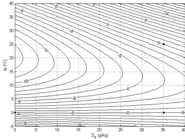
Figure A.19.1. Contours (in °C) of a variable that is used to illustrate the non-conservative production of specific volume. The three points that are forced to be zero are shown with black dots.
